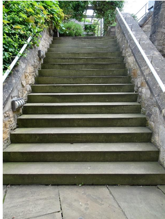
Photo 16 Merifield effective nosings
